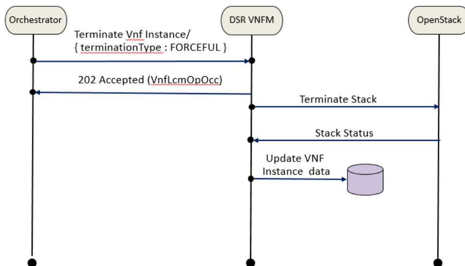
Figure 9. Forceful Termination
