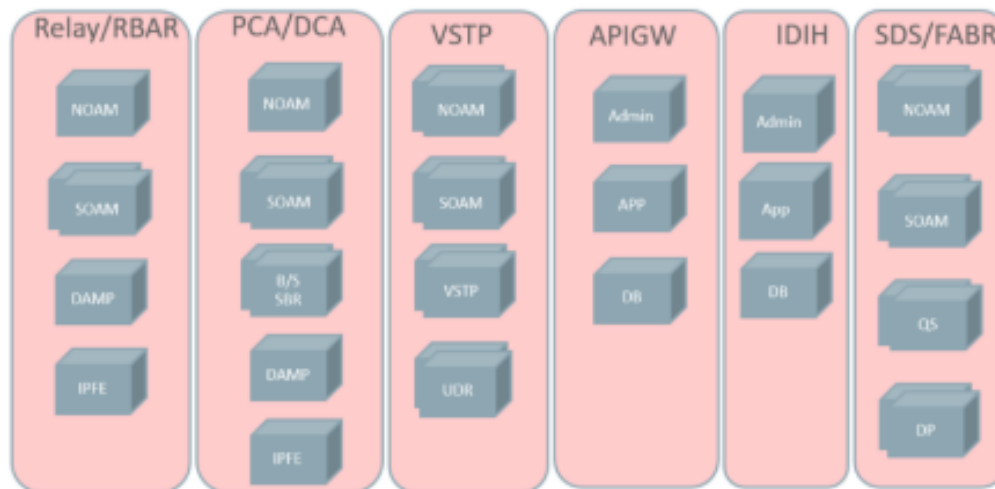
Figure 2. Supported VNFs
