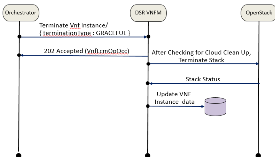
Figure 10. Graceful Termination
